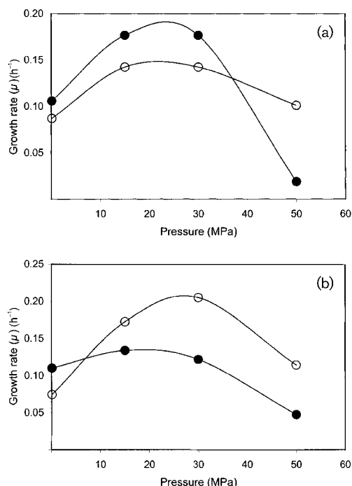
Fig. 3. Growth response of strain 2674 T (a) and strain 2693 T (b) under different pressures at 6 (●) and 10 (○) °C. Growth rates were calculated as described in Fig. 2.
